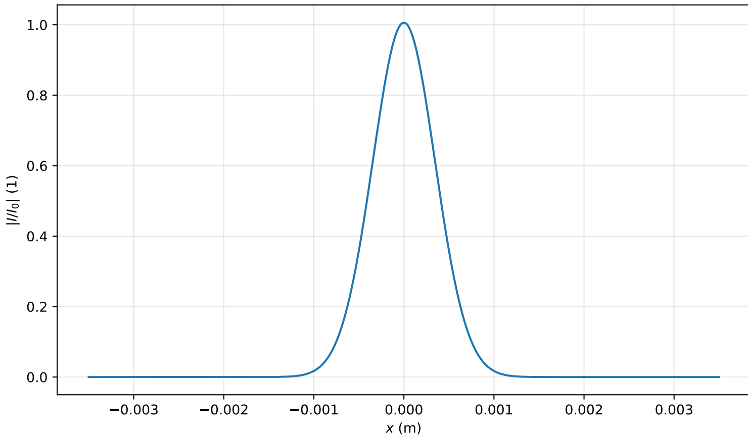
Intensity profile I(x, y = 0, z = 0.159m)/I_0 , P_{in}=0.5P_{cr} , artificial time
